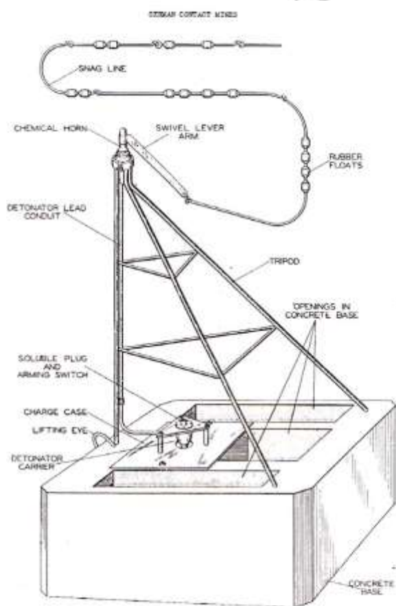
Fig. 14 - Mine Type 0X, elevation
